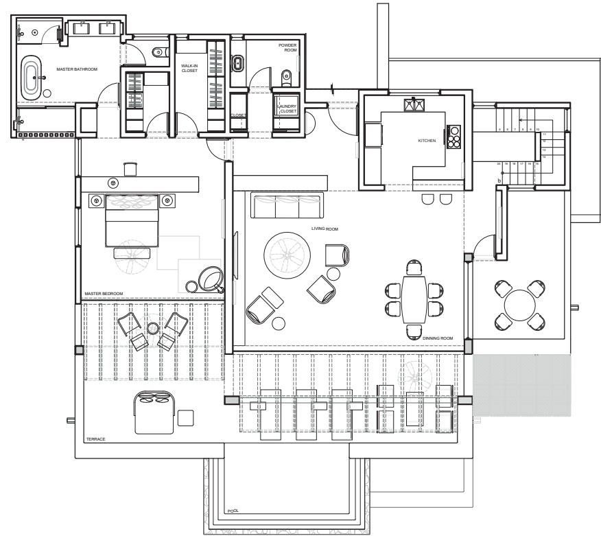
UPPER FLOOR
